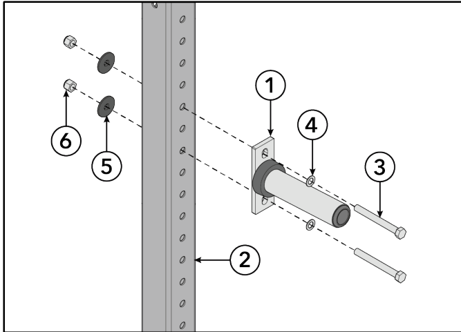
Bumper Plate Configuration
