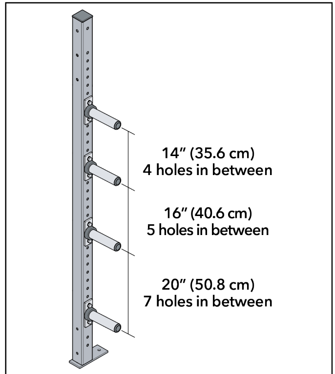
Standard Plate Configuration
