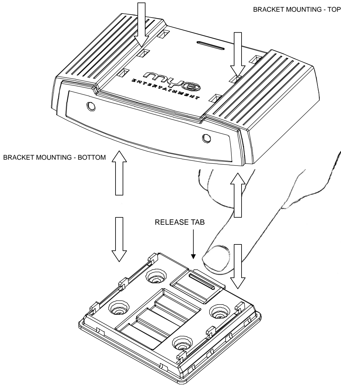
MWT-S9 MOUNTING BRACKET
